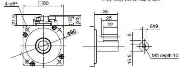
Key way dimensions <Key way, center tap shaft>
